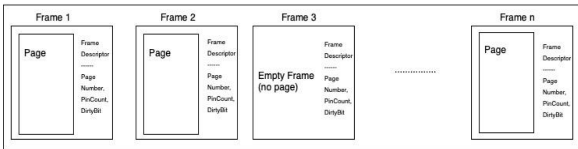
Buffer Pool
