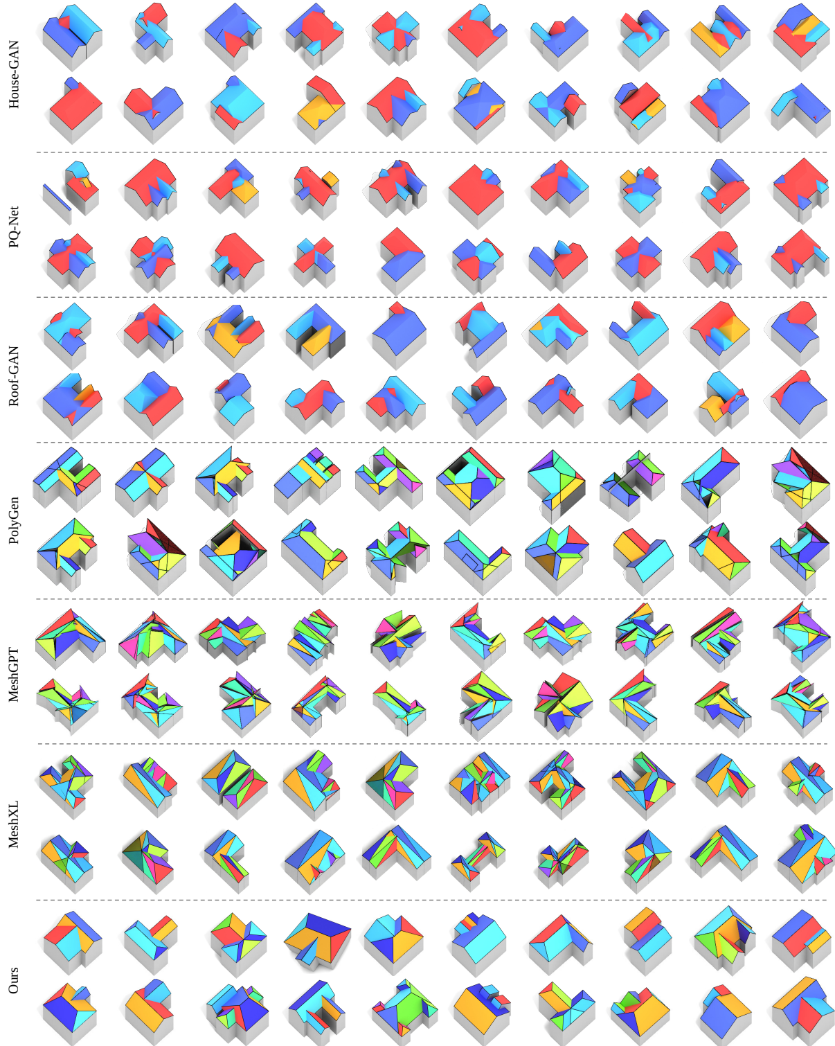
Fig. 9. Visual comparison of generated roof models on the Roof-GAN dataset. Our results demonstrate more complete and geometrically consistent structures. In contrast, the other methods suffer from geometric misalignments and inconsistencies.
