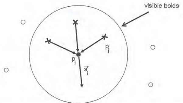
Figure 1. Separation \bar{s}_i is expressed as the sum of all vector corresponding to the oriented lines p_i, p_j . The visible boids are denoted by the cross. The boids not directly visible by the b_i are depicted by the empty circles. The boid b_i is described by the full circle and its position is denoted by p_i .
