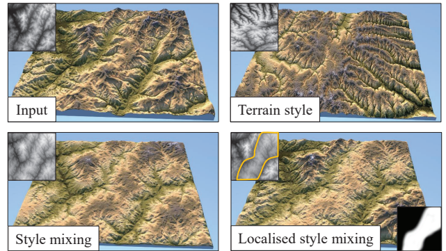
Figure 8: To modify the style over a region \Omega , we run two versions of the generator in parallel, one with \mathbf{f} \in \mathcal{F} extracted from the input and the other from the style. Before invoking the toDEM layer, we blend the feature maps using a user-defined mask derived from \Omega .
