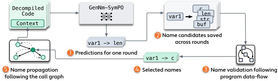
Fig. 7: Inference pipeline of GENNM
