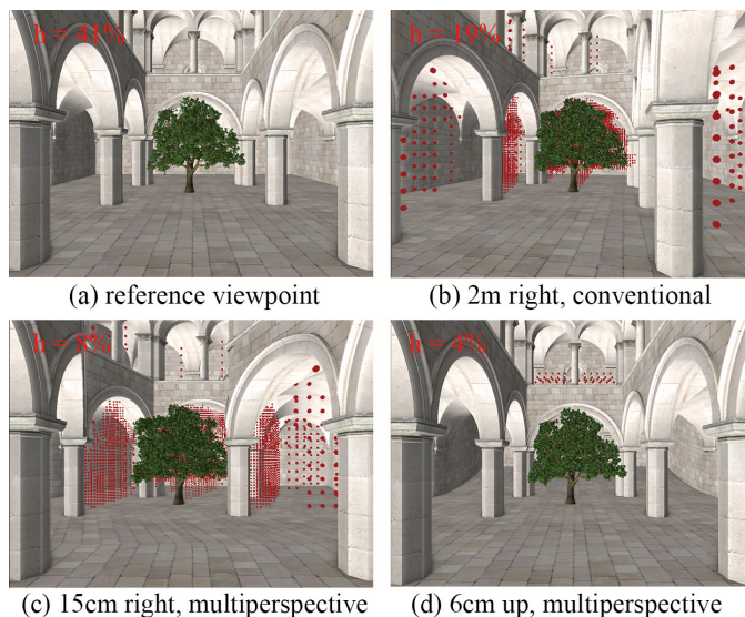
Fig. 2: Occlusion quantification and localization. The pillars and the tree occlude h = 41\% of the VE (a). If the user walks 2m to the right, occlusion is reduced to 19% (b). The disoccluded parts are shown with red dots. Alternatively, with our multiperspective visualization, small head translations efficiently reduce occlusion to 8%, and 4% (c-d).
