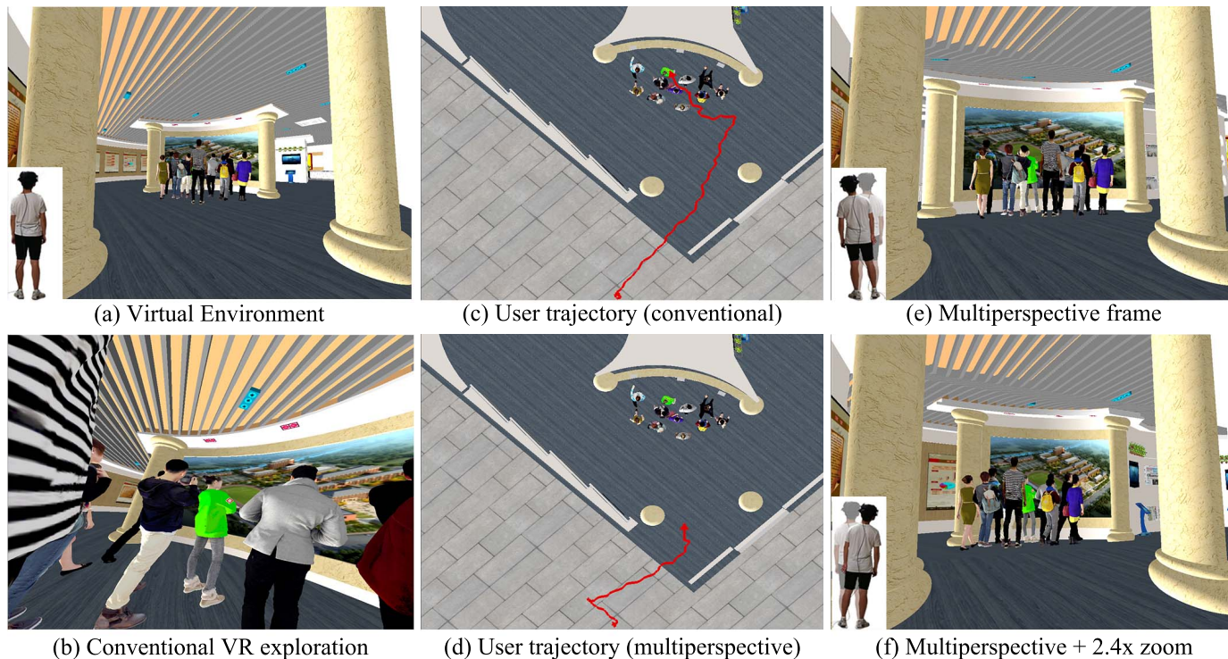
Fig. 1: A user of a VR application is trying to find the person with the green jacket, which is occluded from the current user position (a). With conventional VR exploration, the user has to move closer to the crowd to perform the search (b), which requires significant viewpoint translation (c). With our multiperspective VR exploration technique, the user can search the crowd from the current position (e), with an intuitive lateral head translation, which makes the exploration of the virtual environment more efficient (d). The user can also zoom in on the crowd for greater detail (f). Nearby geometry (e.g. nearby pillars) is rendered from the original user perspective at all times, anchoring the user to prevent disorientation and simulation sickness (e, f).
