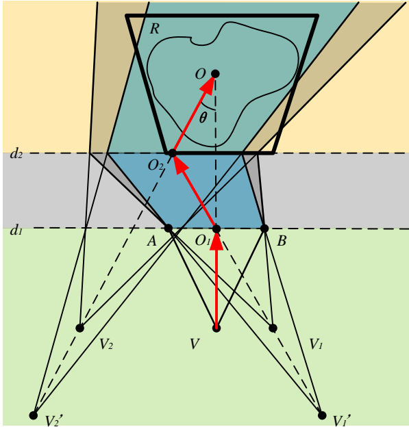
Fig. 7: Two-bend graph camera construction for fine-grain disocclusion of region R . Secondary viewpoints V_1 and V_2 allow changing the view direction on R by angle \theta , while keeping the projection of center O of R in place. Nearby geometry is rendered with the original viewpoint V (green), anchoring the user. When the secondary viewpoints V_1 and V_2 are moved back to V_1' and V_2' , image region AB is mapped to a smaller VE region (blue), which produces a magnification effect.
