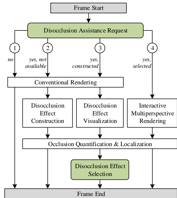
Fig. 3: Overview of our method for occlusion removal assistance.
